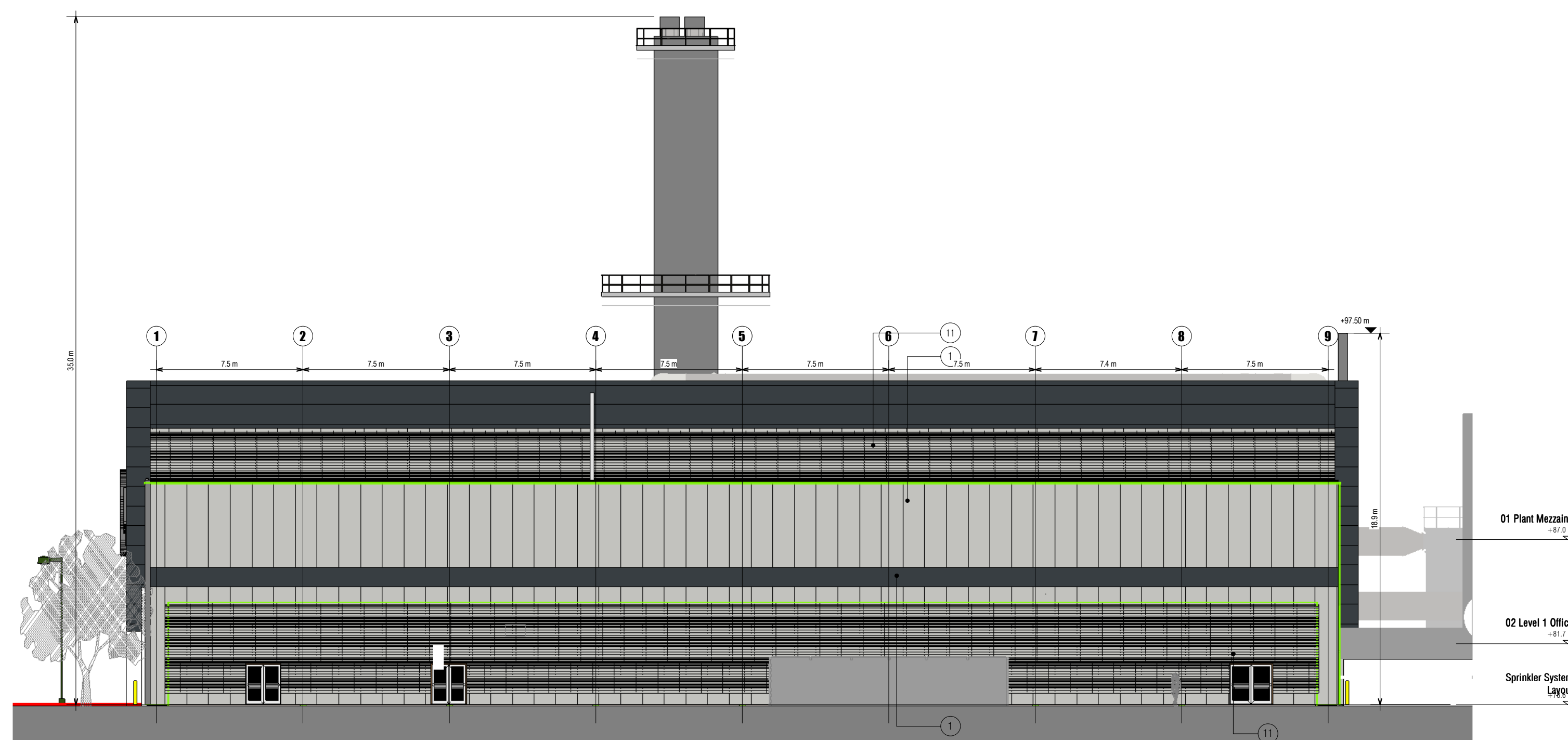
2 West Elevation 1 : 200
