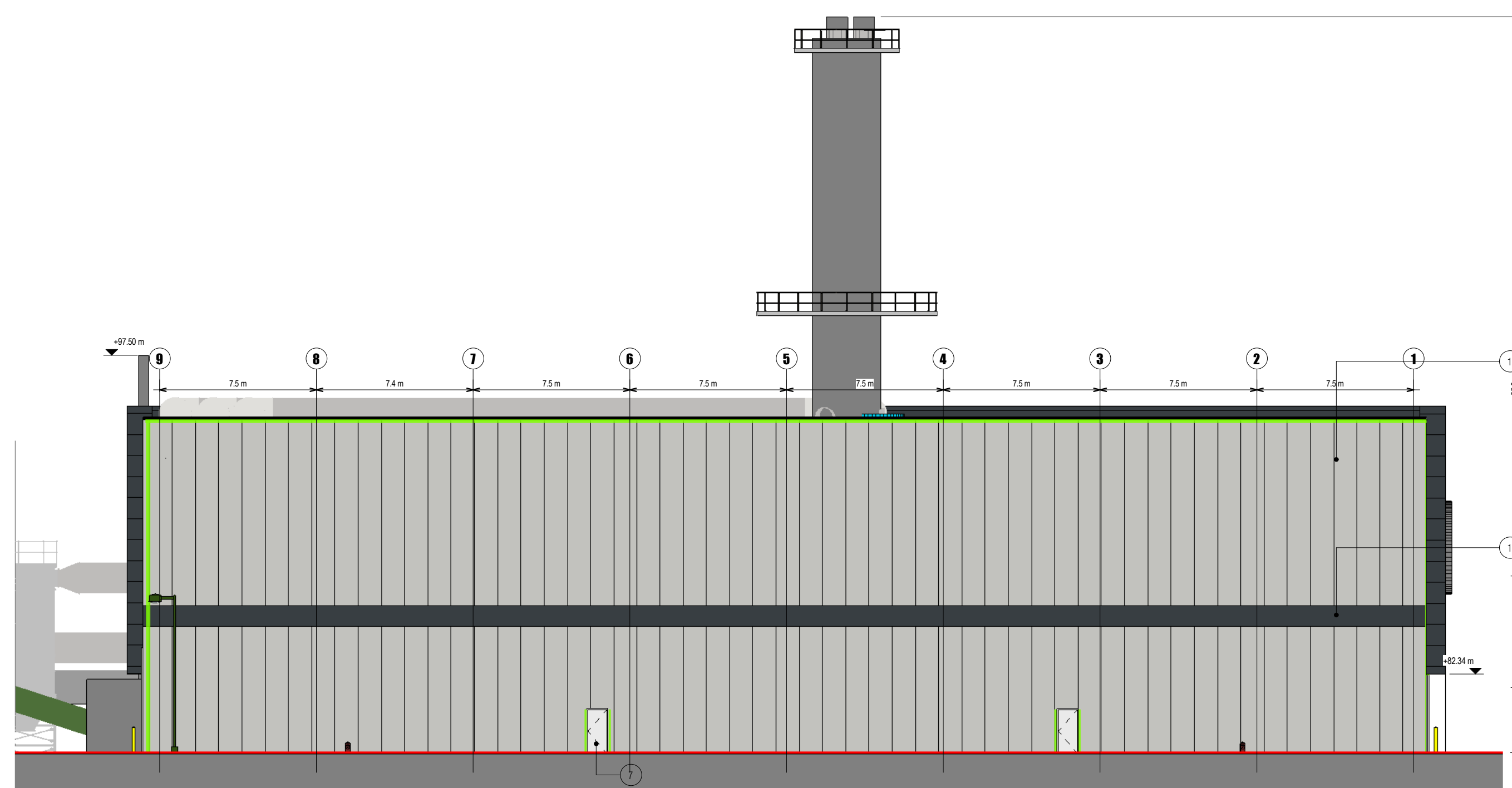
1 East Elevation 1:200
